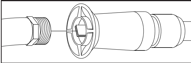
Figure 15 — Backflushing the Nozzle
